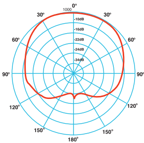
HIGHLY DIRECTIONAL POLAR RESPONSE
